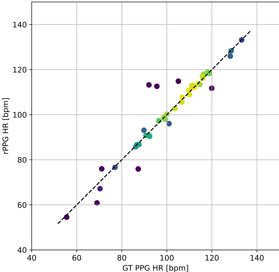
UBFC_UBFC_physnet_FFT_BlandAltman_ScatterPlot
